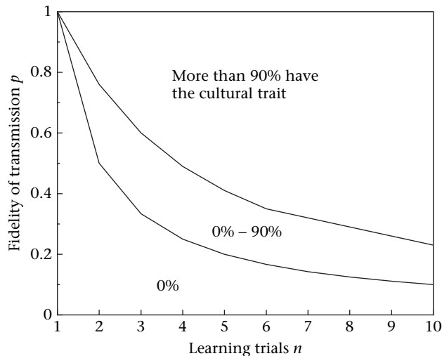
Figure 2. The diagram shows how combinations of the number ( n ) of learning trials and the fidelity of social learning ( p ) promote different equilibrium frequencies ( x_\infty ). Each learning trial uses a new cultural parent drawn at random from the parent population (see text).
